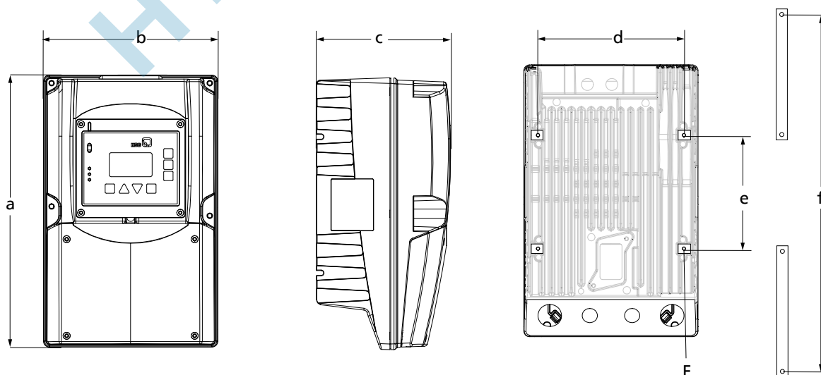
III. 3: Dimensions PumpDrive 2 Eco
