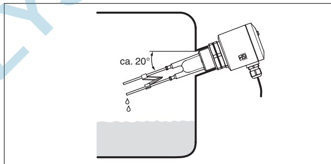
Fig. 6: Montage horizontal
