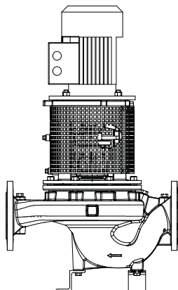
III. 7: Installation verticale, Etaline SYT
