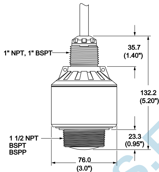
Figure 12.1 Encombrement SITRANS LR100
