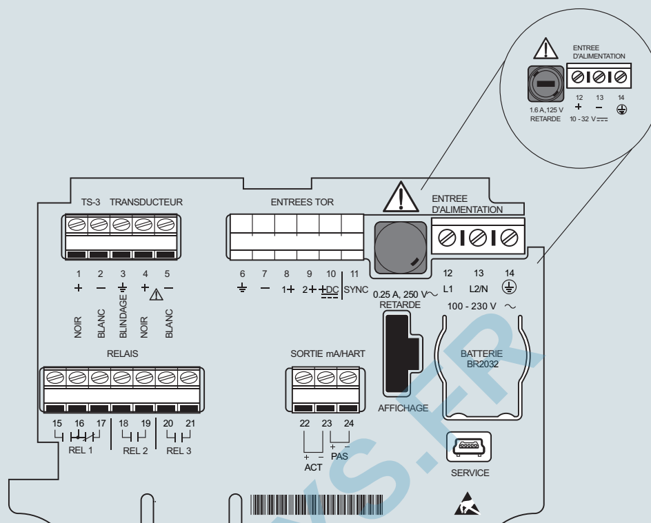
SITRANS LUT400 raccords
