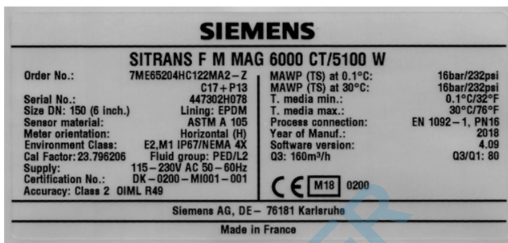
Figure 2-2 Plaque signalétique du MAG 6000, 5100 W
