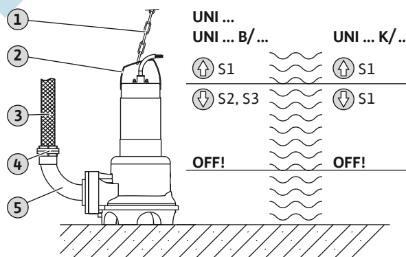
Fig. 6: Installation immergée transportable
