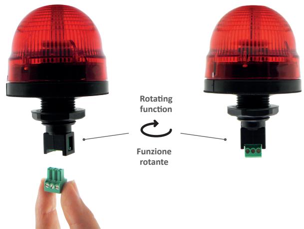
Removable screw cable clamp Morsetteria estraibile
