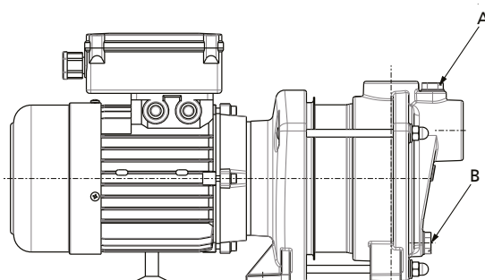
III. 10: Orifices
