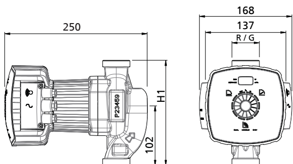
III. 7: Dimensions Calio S BMS [mm]
