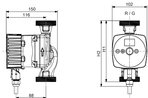
III. 6: Dimensions Calio S Pro [mm]
