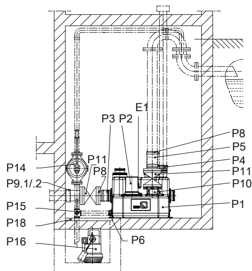
III. 20: mini-Compacta U (60 litres)
