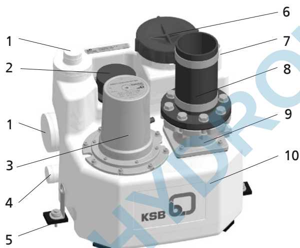
III. 1: Photo station de relevage
