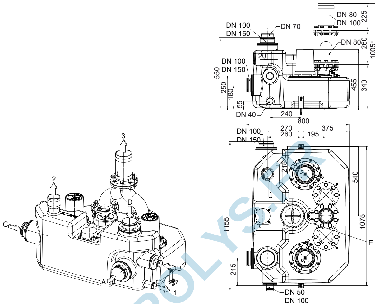
III. 9: Raccordements et dimensions mini-Compacta UZ (150 litres)
