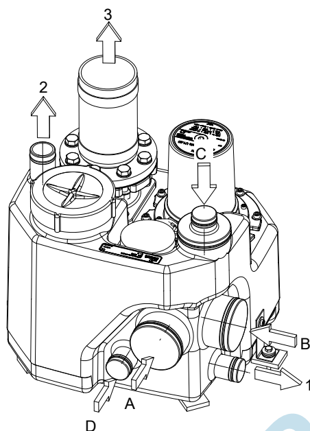
III. 6: Raccordements et dimensions mini-Compacta U (60 litres)
