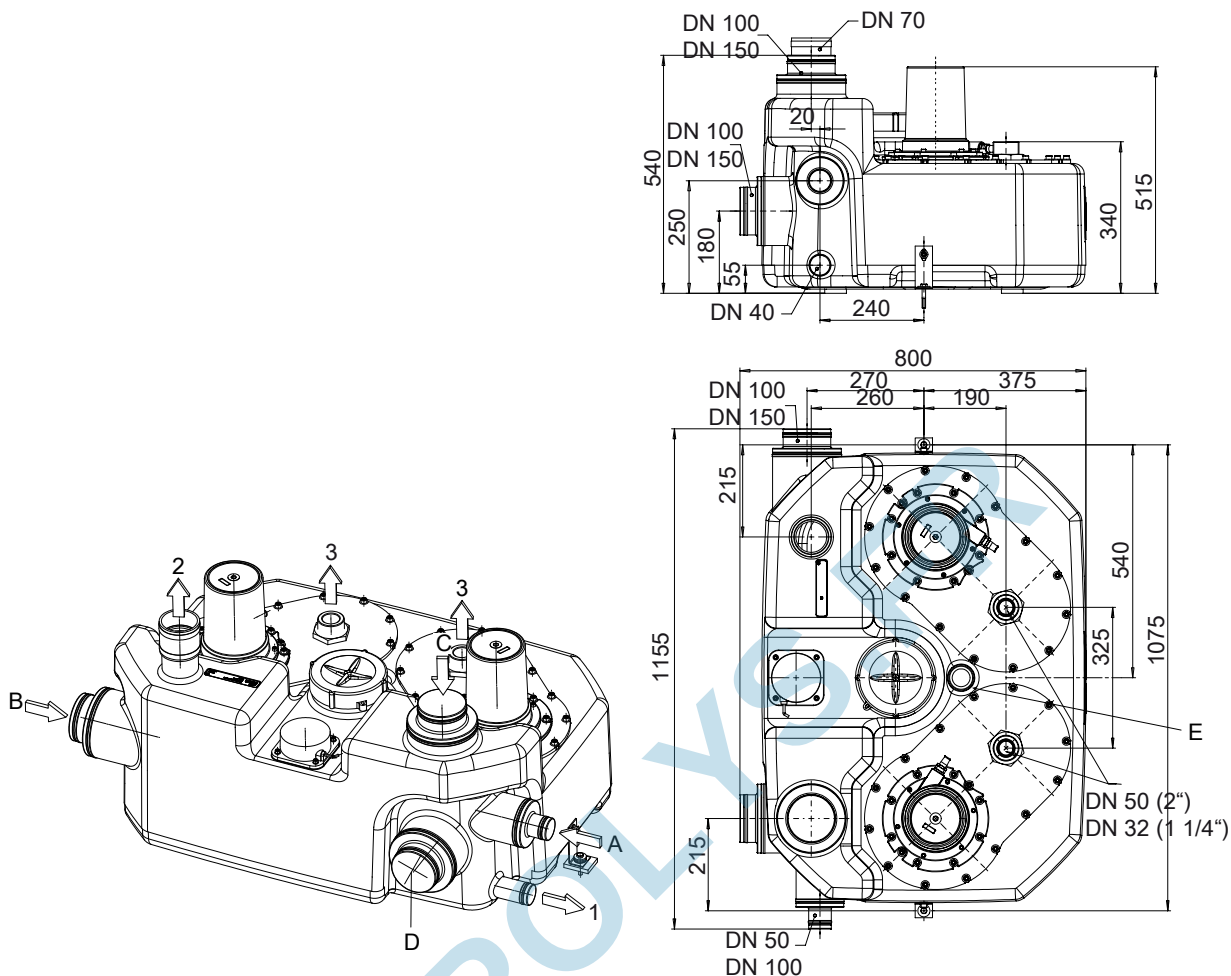
III. 10: Raccordements et dimensions mini-Compacta UZS (150 litres)
