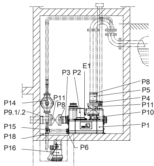
III. 23: mini-Compacta U (100 litres)
