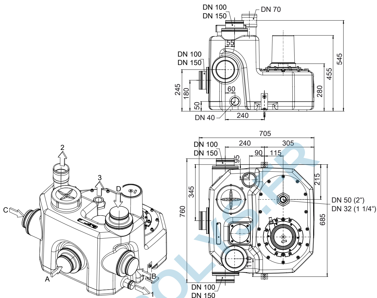
III. 8: Raccordements et dimensions mini-Compacta US (100 litres)
