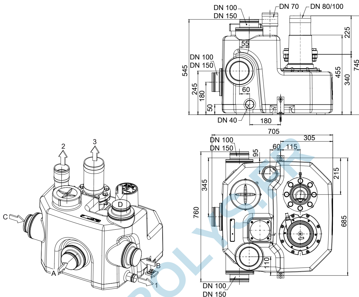
III. 7: Raccordements et dimensions mini-Compacta U (100 litres)
