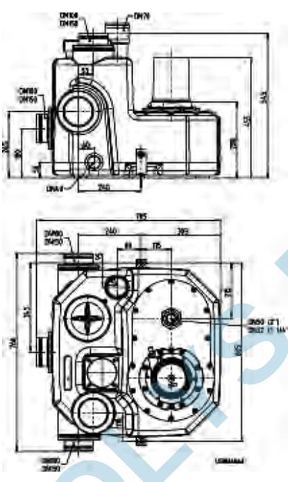
mini-Compacta U100
