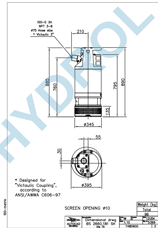
Figure 15: BS, SH, DN 75
