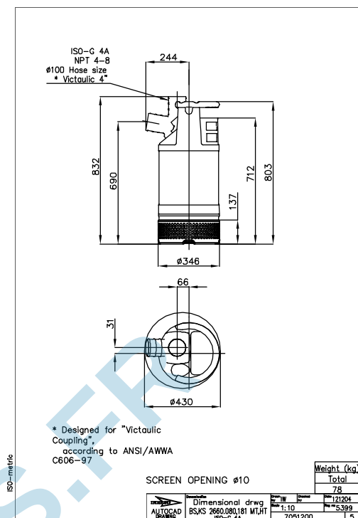
Figure 11: BS/KS, MT/HT, DN 100
