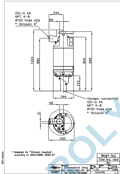
Figure 8: BS, MT, DN 100, tandem
