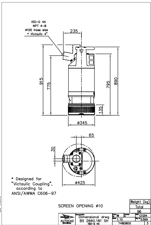
Figure 16: BS, SH, DN 100
