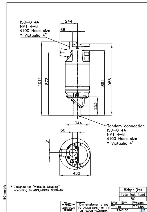
Figure 14: BS, HT, DN 100, tandem
