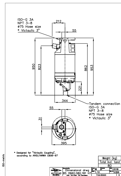
Figure 13: BS, HT, DN 75, tandem
