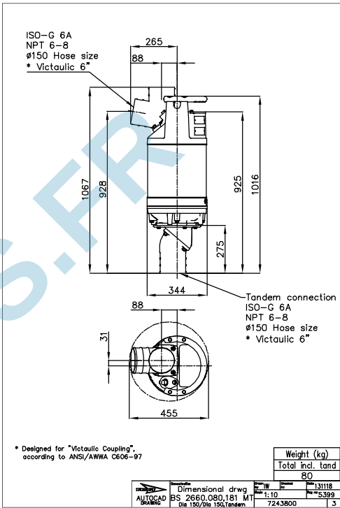
Figure 9: BS, MT, DN 150, tandem
