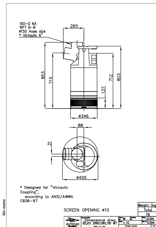
Figure 10: BS/KS, MT, DN 150
