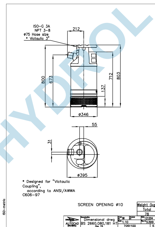
Figure 12: BS, HT, DN 75
