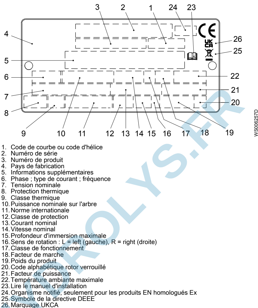
Figure 1: Plaque signalétique
