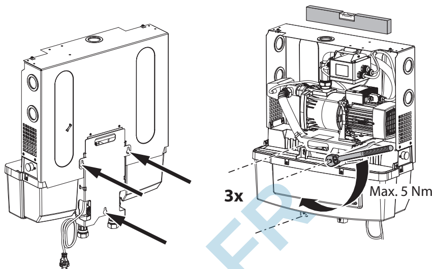
Fig. 13: Fixation points for wall suspension and tightening the screws
