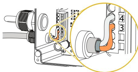
Fig. 18: Screwed connection
