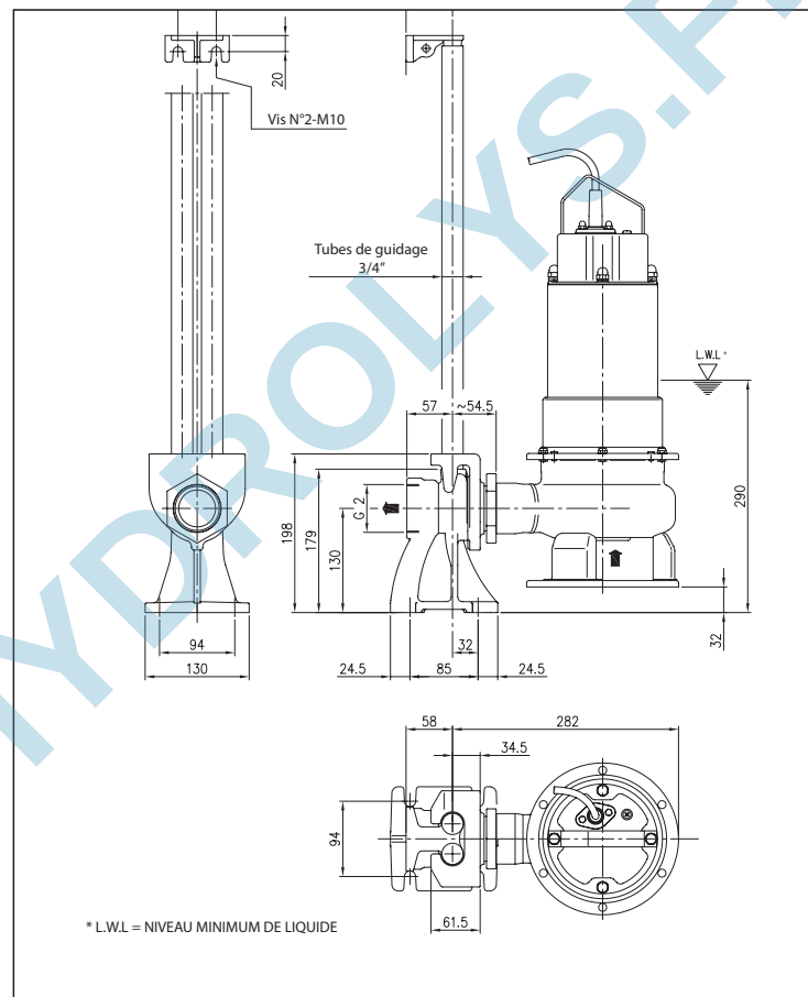
DIMENSIONS KIT ACCOUPLEMENT DW-DW VOX
