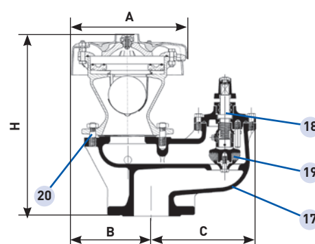
Vannair V1000 ARA
