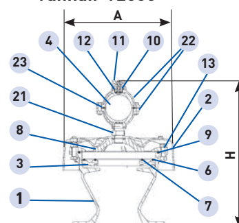
Vannair V2000
