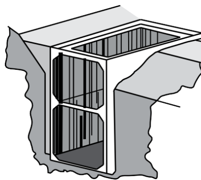
Figure 3 : Blindage excavation
