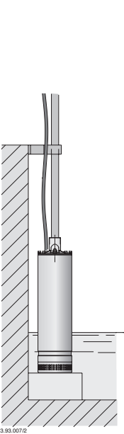
Fig. 1 Pompa appoggiata Pump in the standing position Pompe posée
